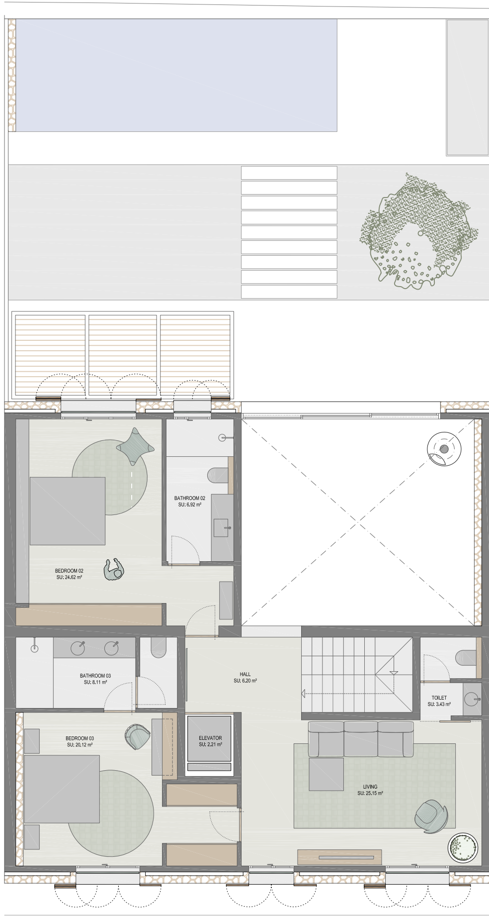
- OLIVO II - FIRST FLOOR
